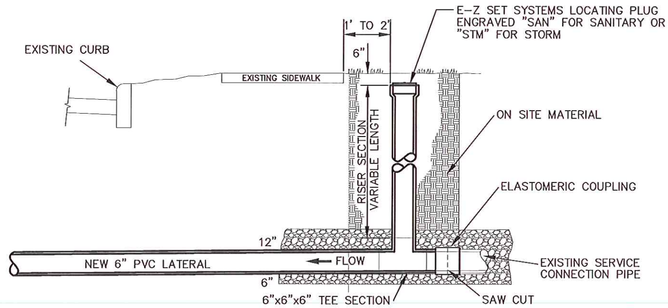
INSPECTION TEE IN LAWN AREA SANITARY OR STORM
