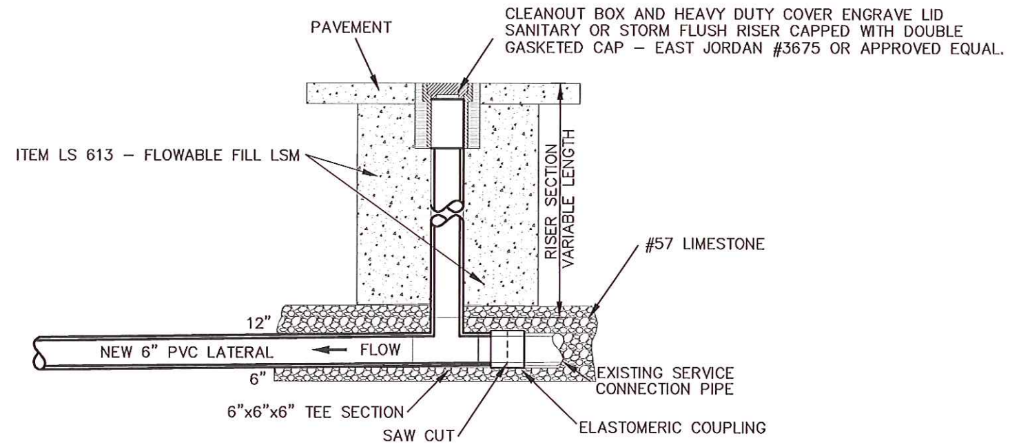
INSPECTION TEE IN PAVEMENT SANITARY OR STORM
