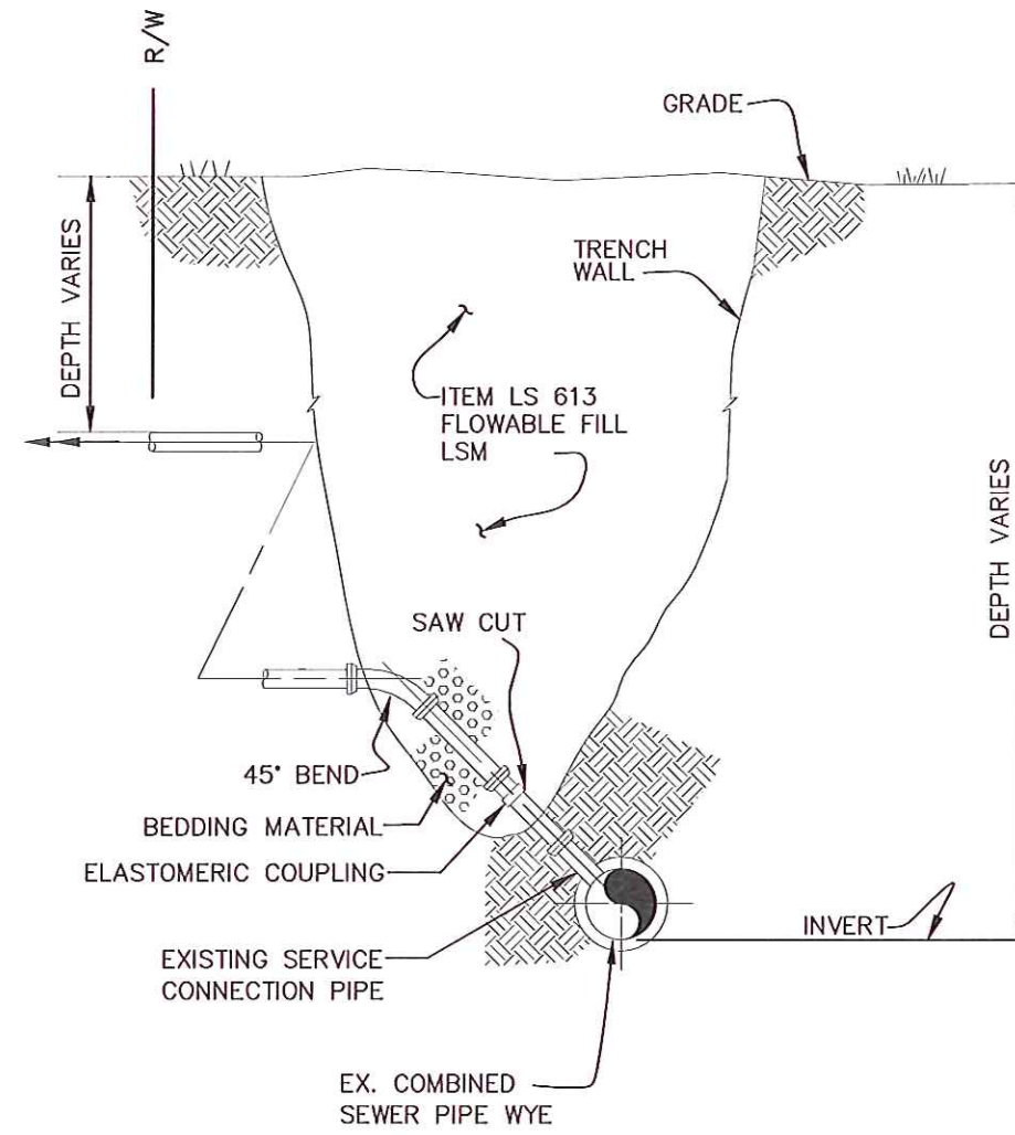
SECTION NEW SERVICE CONNECTION TO EXISTING SEWER MAIN
