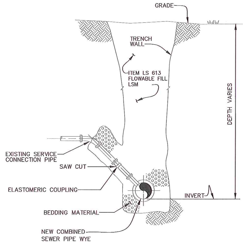
SECTION EXISTING SERVICE CONNECTION TO NEW SEWER MAIN
